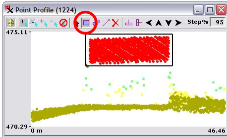
LIDAR points marked using the Rectangle tool in the Point Profile. Marked points (red in this illustration) are also marked in the View (illustration to the right). The shape of this point set in profile and plan views indicates that these points represent the pitched roof of a rectangular building.
