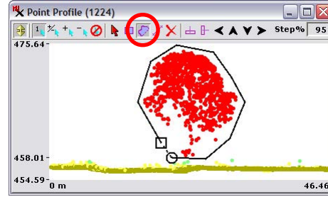
LIDAR points marked using the Polygon tool in the Point Profile. Marked points (red in this illustration) are also marked in the View (illustration to the right). The globular shape of this point set in profile and plan views and its height above the ground surface indicates that most of the marked points are returns from the foliage and branches of a tree.
