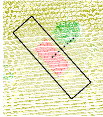
LIDAR points marked using the Rectangle tool in the Point Profile. Marked points (red in this illustration) are also marked in the View (illustration to the right). The shape of this point set in profile and plan views indicates that these points represent the pitched roof of a rectangular building.
