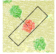
LIDAR points marked using the Polygon tool in the Point Profile. Marked points (red in this illustration) are also marked in the View (illustration to the right). The globular shape of this point set in profile and plan views and its height above the ground surface indicates that most of the marked points are returns from the foliage and branches of a tree.
